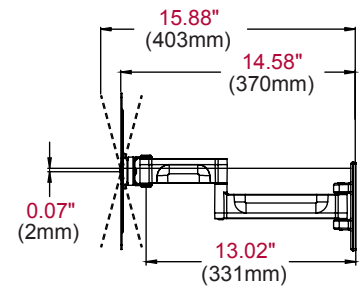
SIDE VIEW EXTENDED +/- 15° TILT
